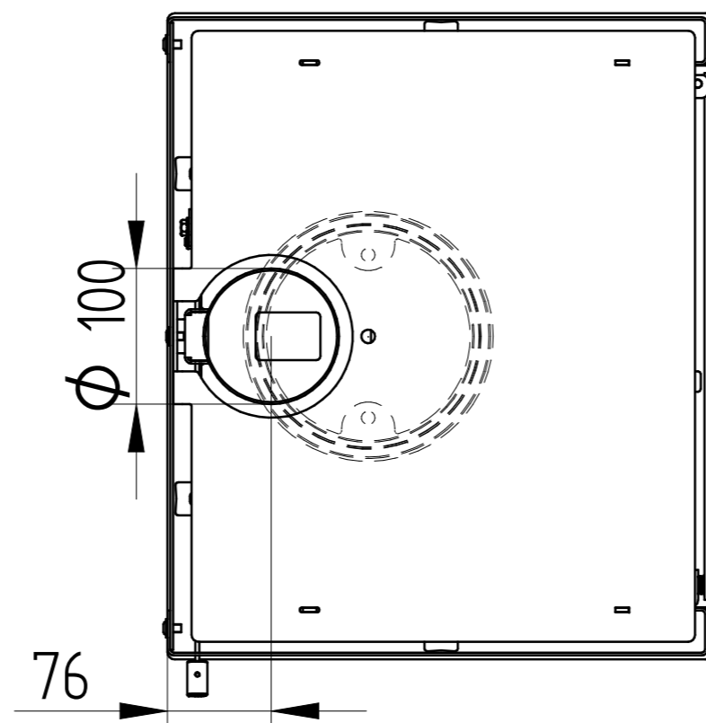
SECTION E-E
